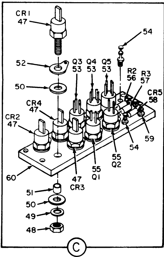
Figure 6. LNA power supply assembly (sheet 2 of 2 sheets).
