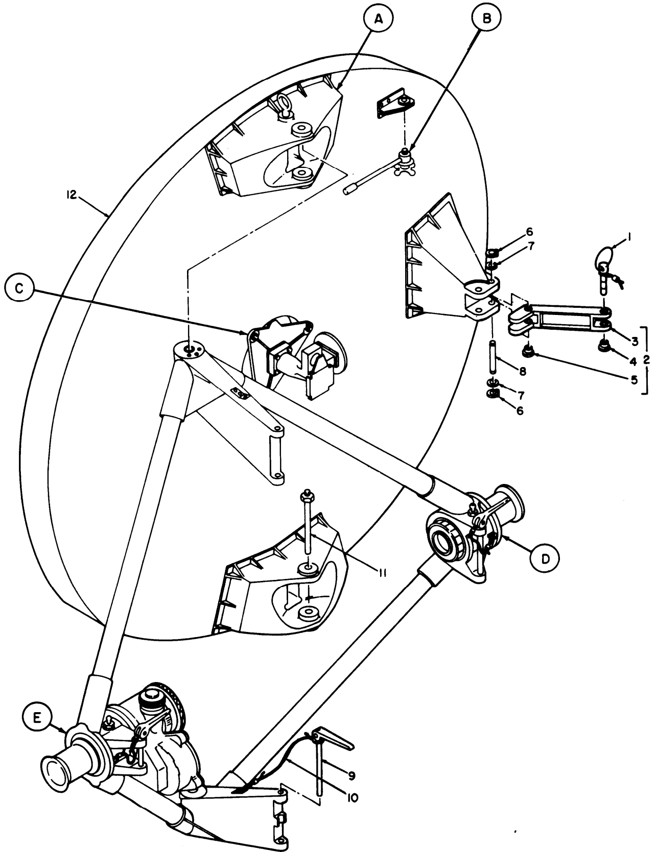
Figure 15. Reflector gimbal assembly (sheet 1 of 8 sheets).
