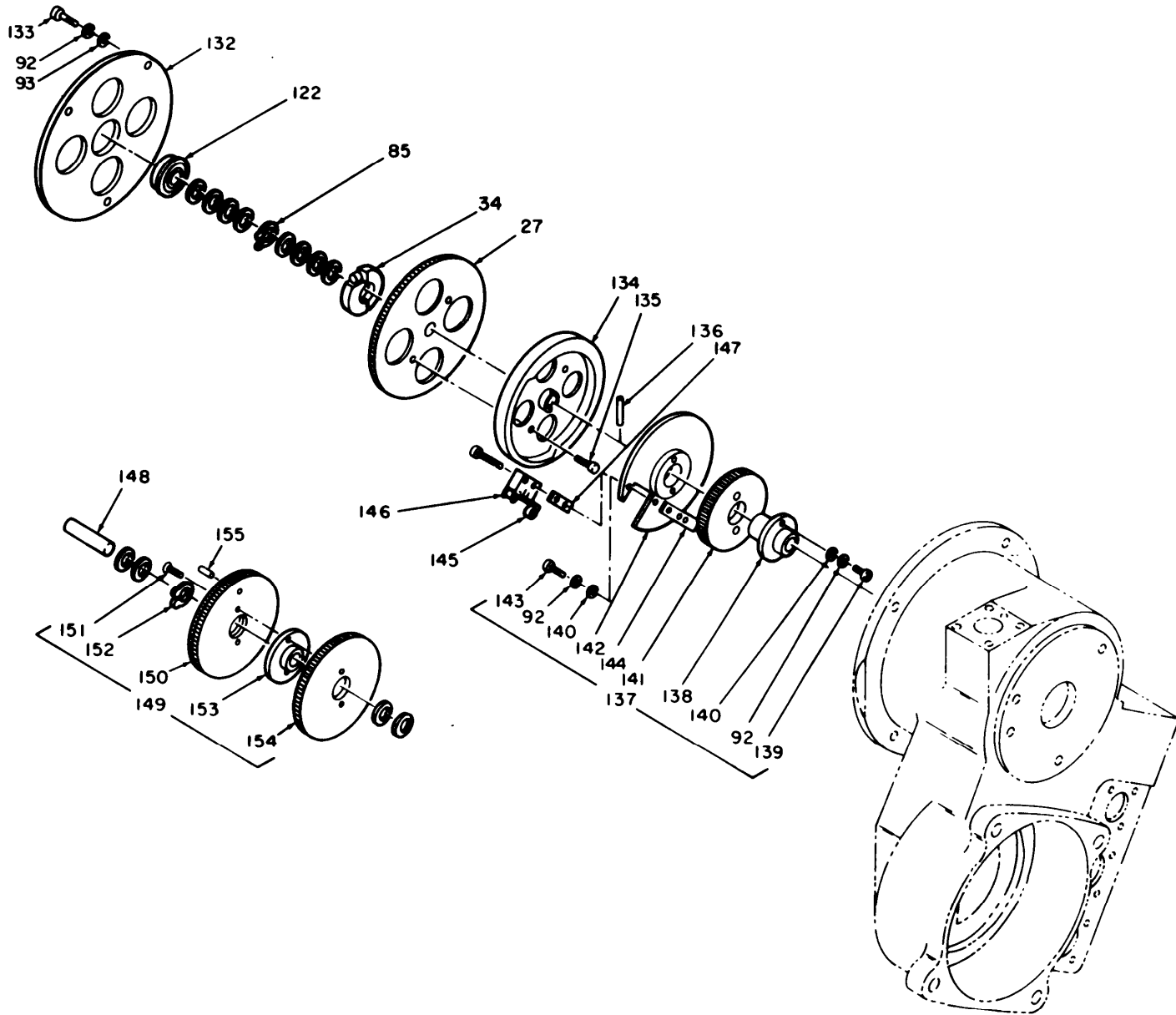
Figure 15. Reflector gimbal assembly (sheet 8 of 8 sheets).
