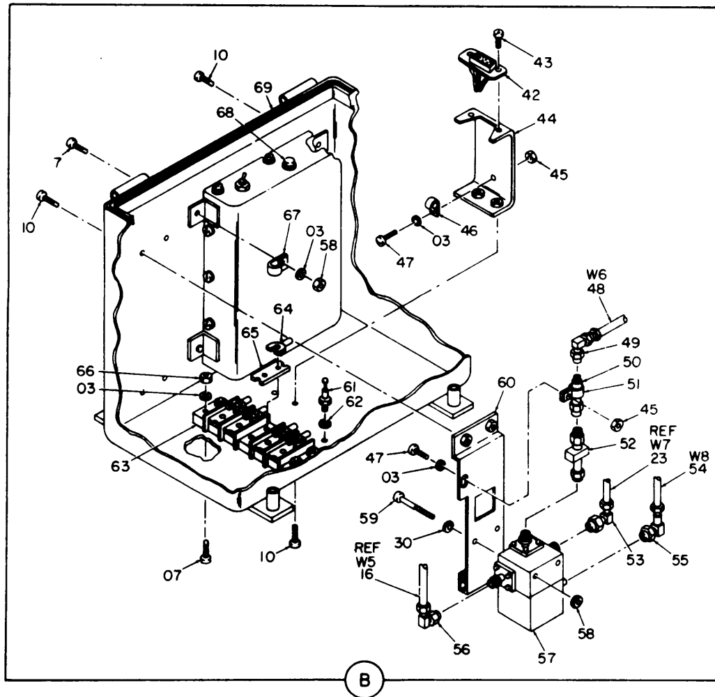
Figure 9. LNA BITE assembly (sheet 2 of 2 sheets).
