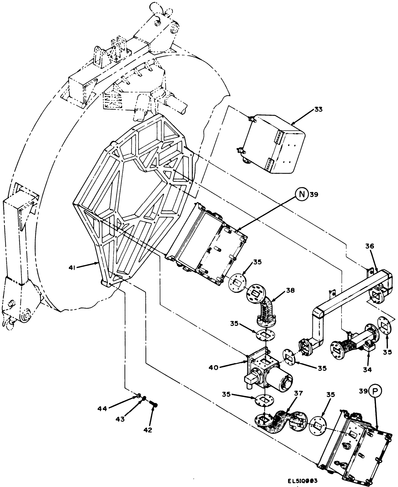
Figure 1. Antenna mounted electronics (sheet 3 of 4 sheets).
