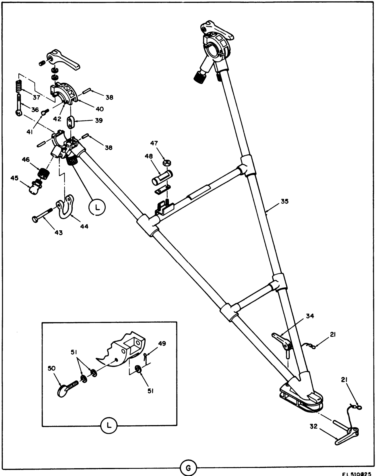
Figure 12. Antenna AS-3036/TSC (sheet 6 of 7 sheets).
