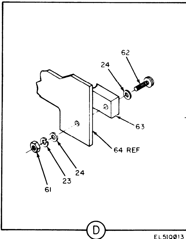
Figure 6. LNA power supply assembly (sheet 2 of 2 sheets).
