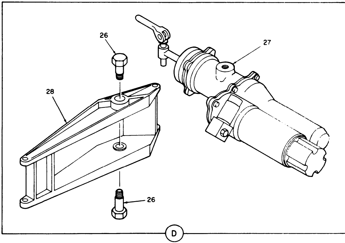
Figure 12. Antenna AS-3036/TSC (sheet 3 of 7 sheets.)
