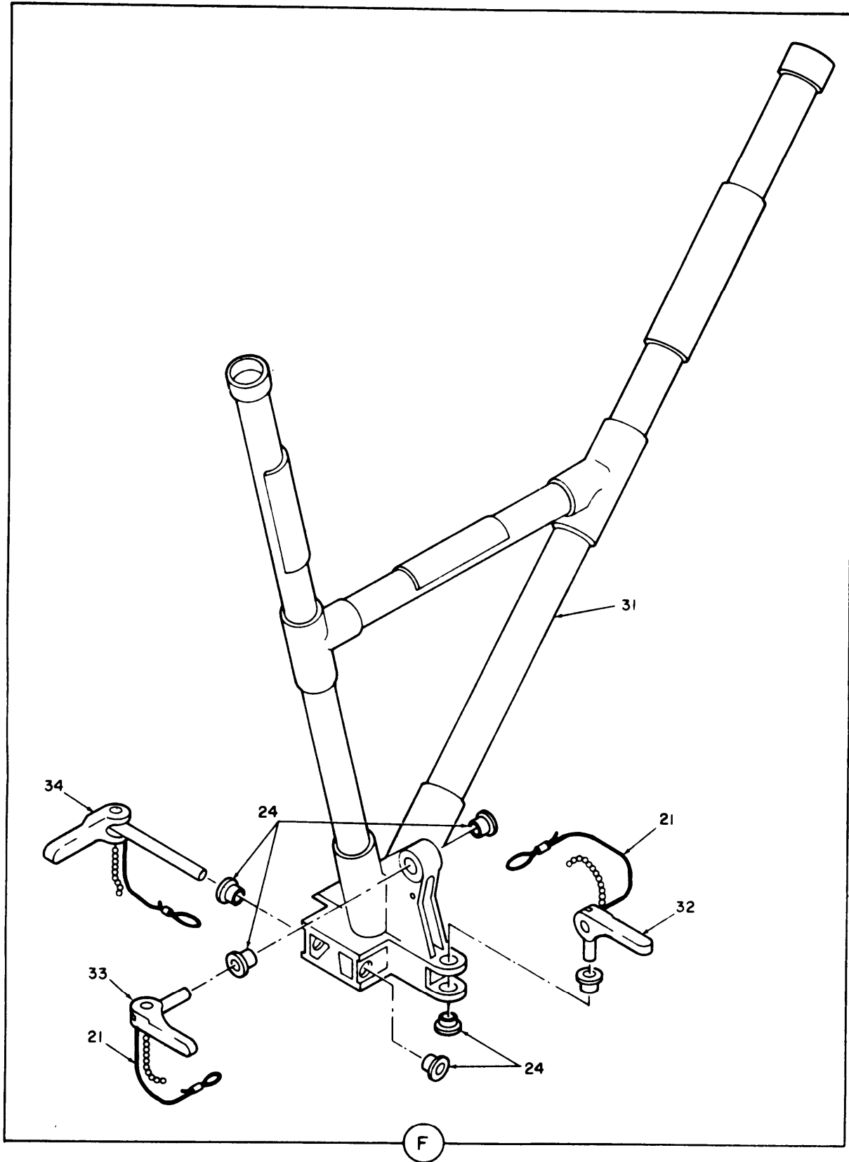
Figure 12. Antenna AS-3036/TSC (sheet 5 of 7 sheets).
