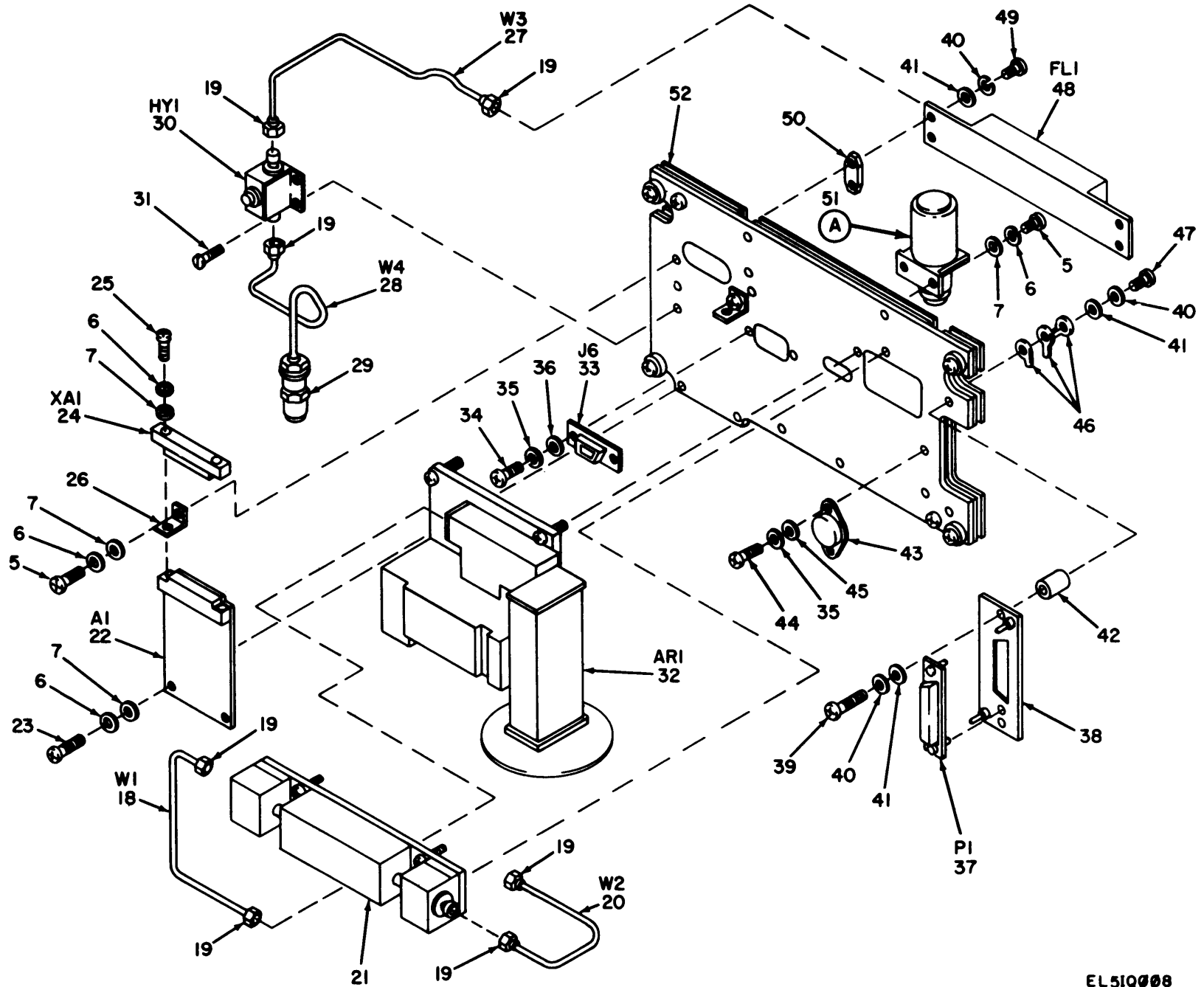
Figure 3. RF amplifier assembly (sheet 3 of 4 sheets).
