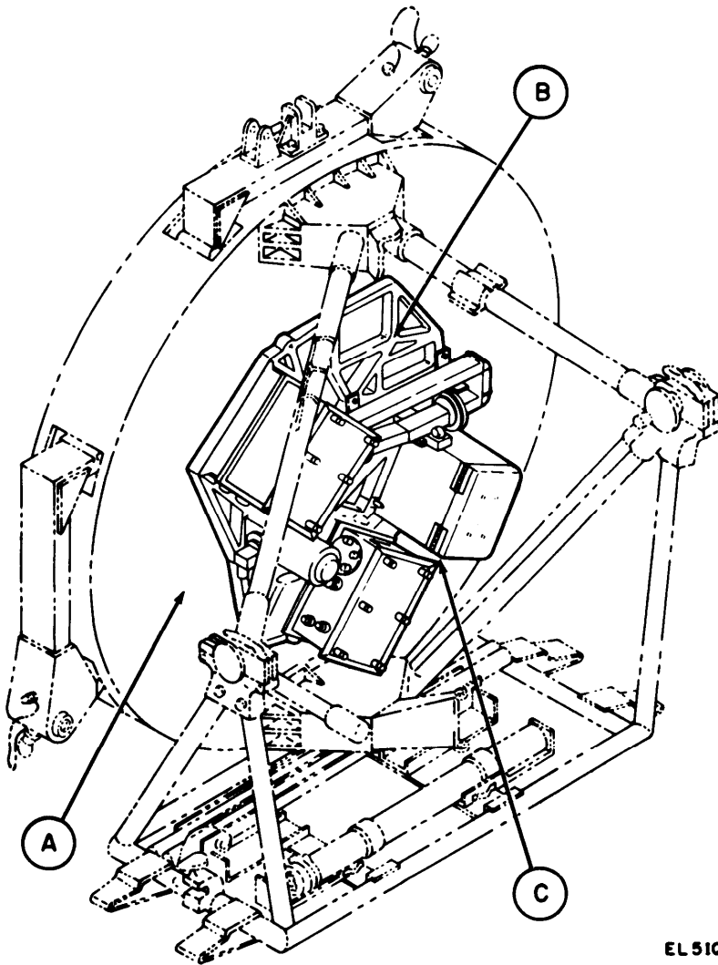
Figure 1. Antenna mounted electronics (sheet 1 of 4 sheets).
