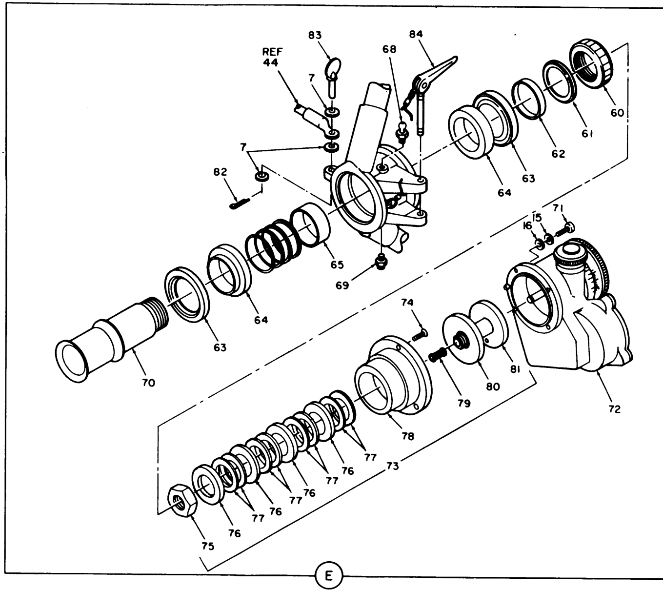
Figure 15. Reflector gimbal assembly (sheet 6 of 8 sheets).
