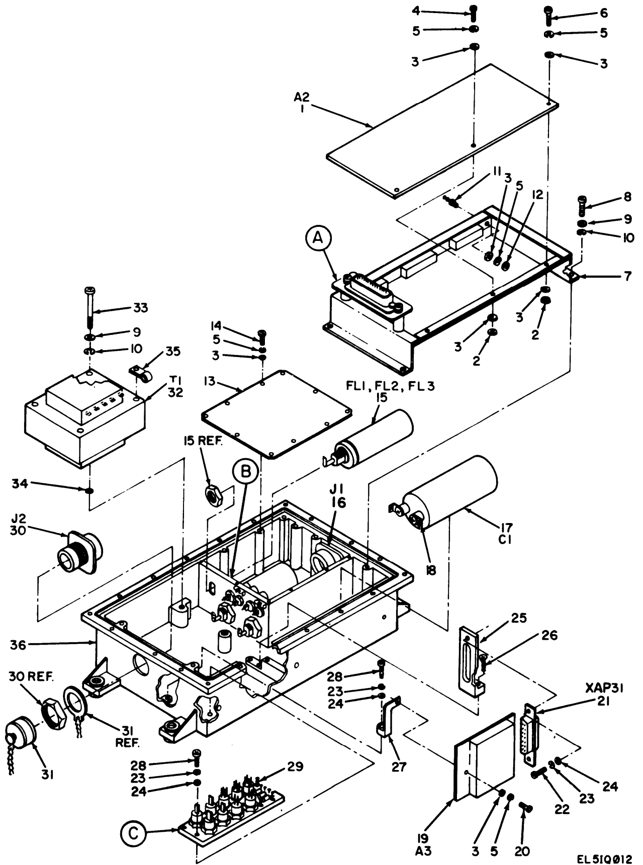
Figure 6. LNA power supply assembly (sheet 1 of 2 sheets).
