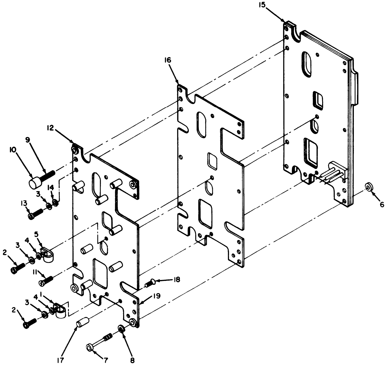
Figure 5. Heater plate.
